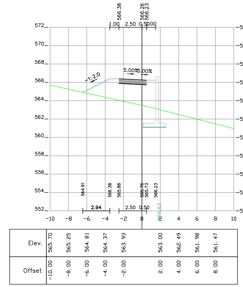
1+400 [Road road-3]
