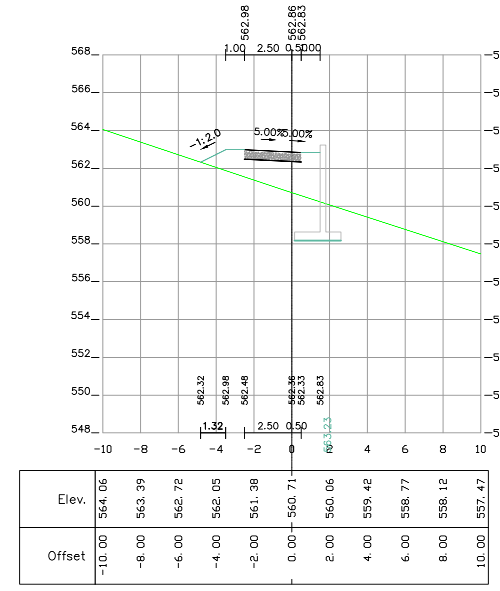
1+380 [Road road-3]
