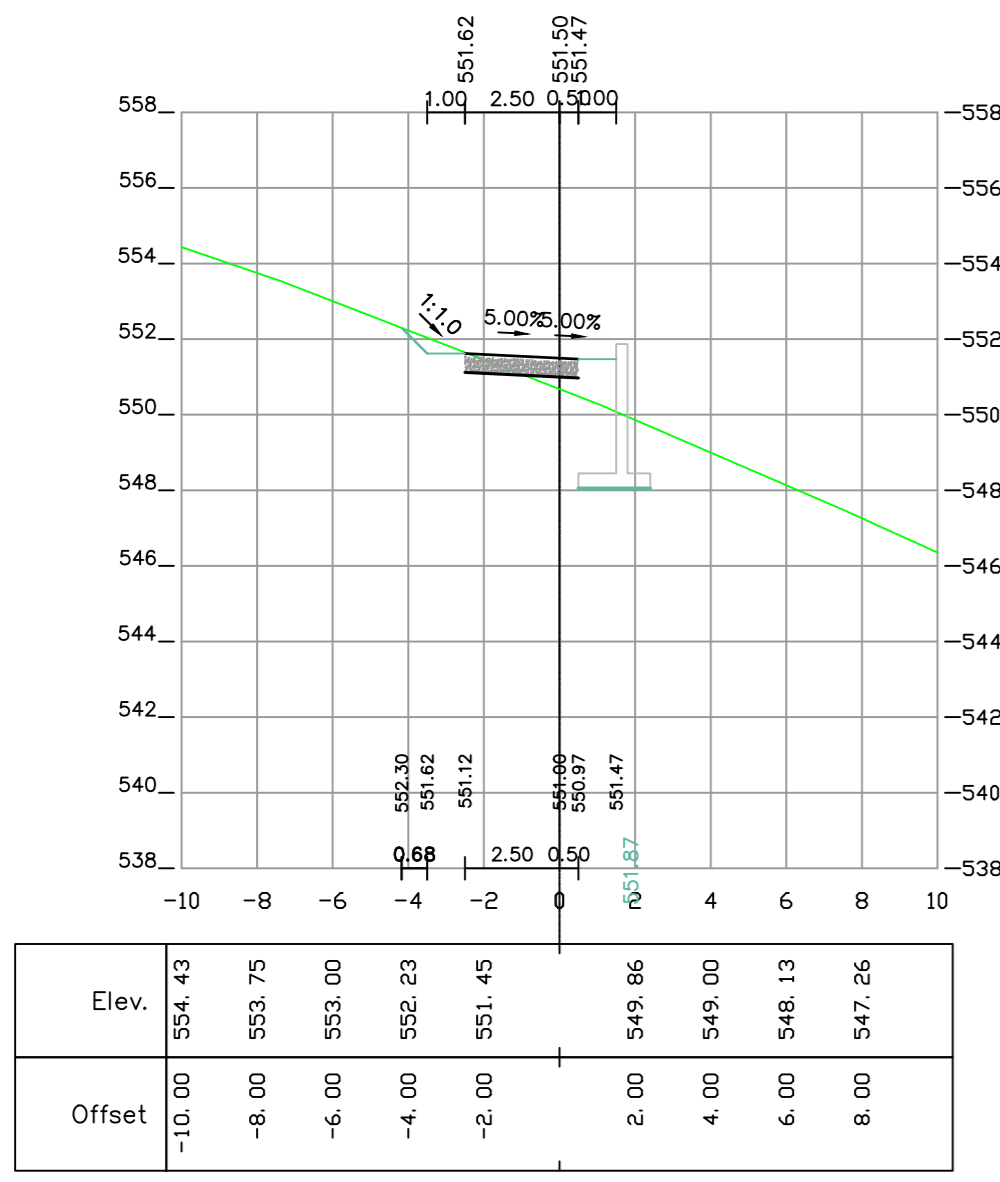
1+160 [Road road-3]
