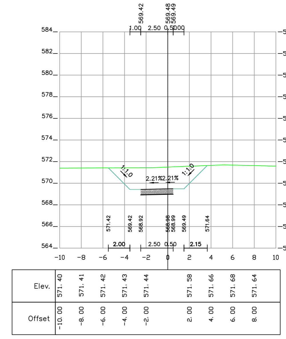
1+440 [Road road-3]
