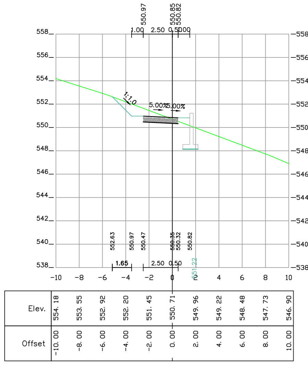
1+140 [Road road-3]
