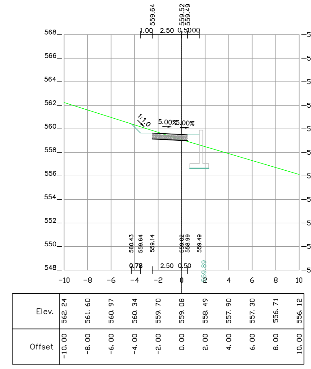
1+360 [Road road-3]
