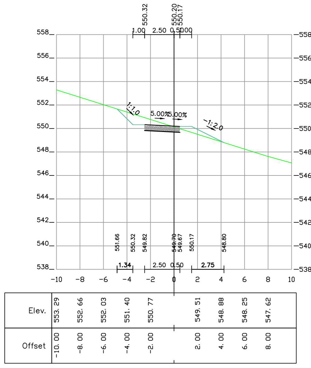
1+120 [Road road-3]
