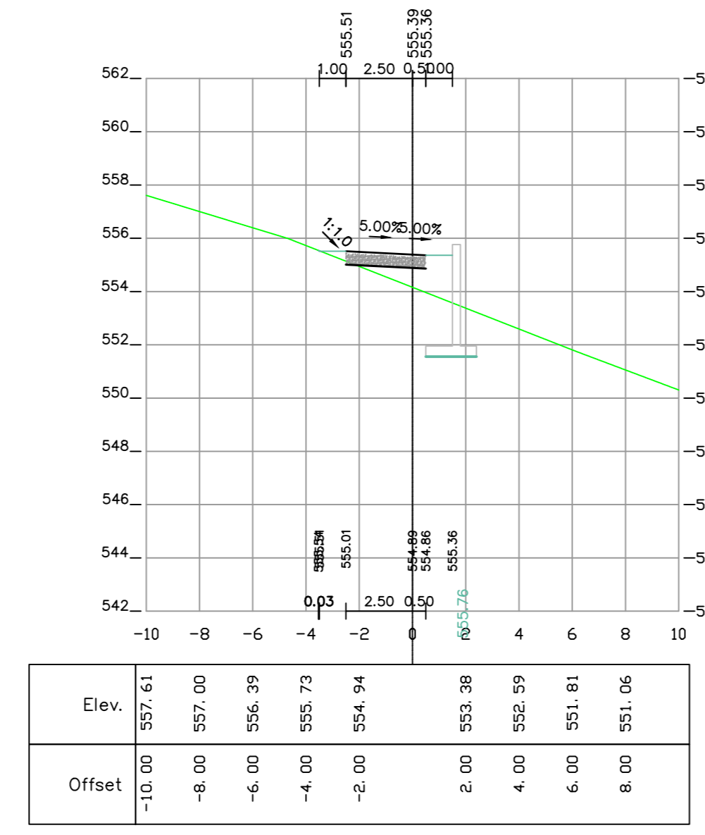
1+280 [Road road-3]
