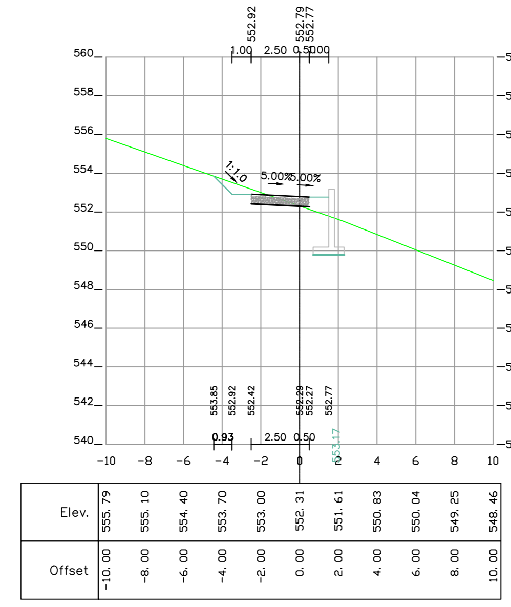
1+200 [Road road-3]
