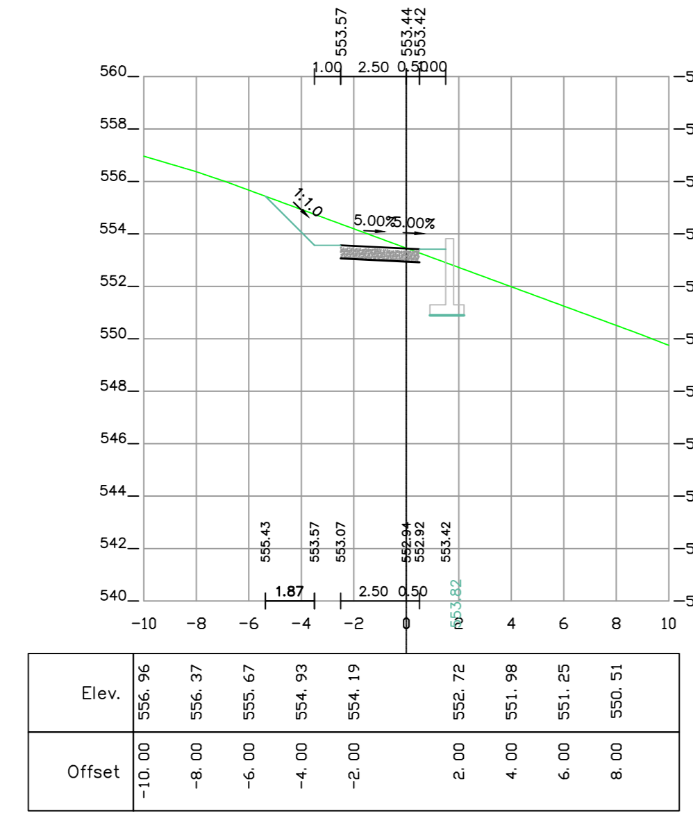
1+220 [Road road-3]
