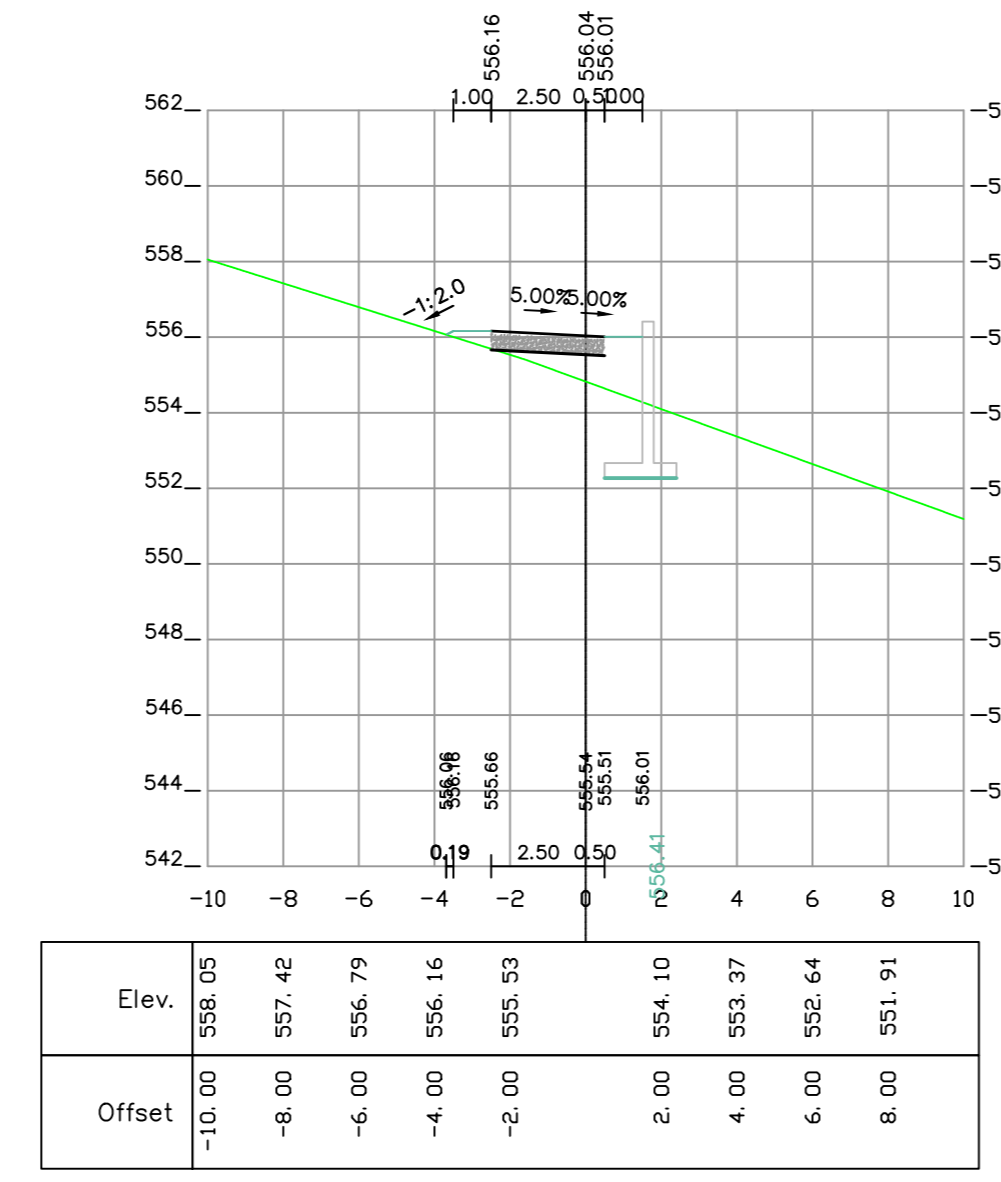
1+300 [Road road-3]
