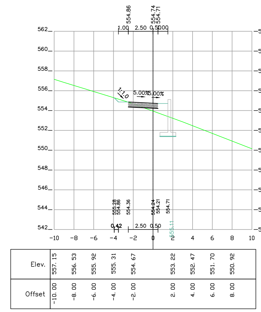
1+260 [Road road-3]
