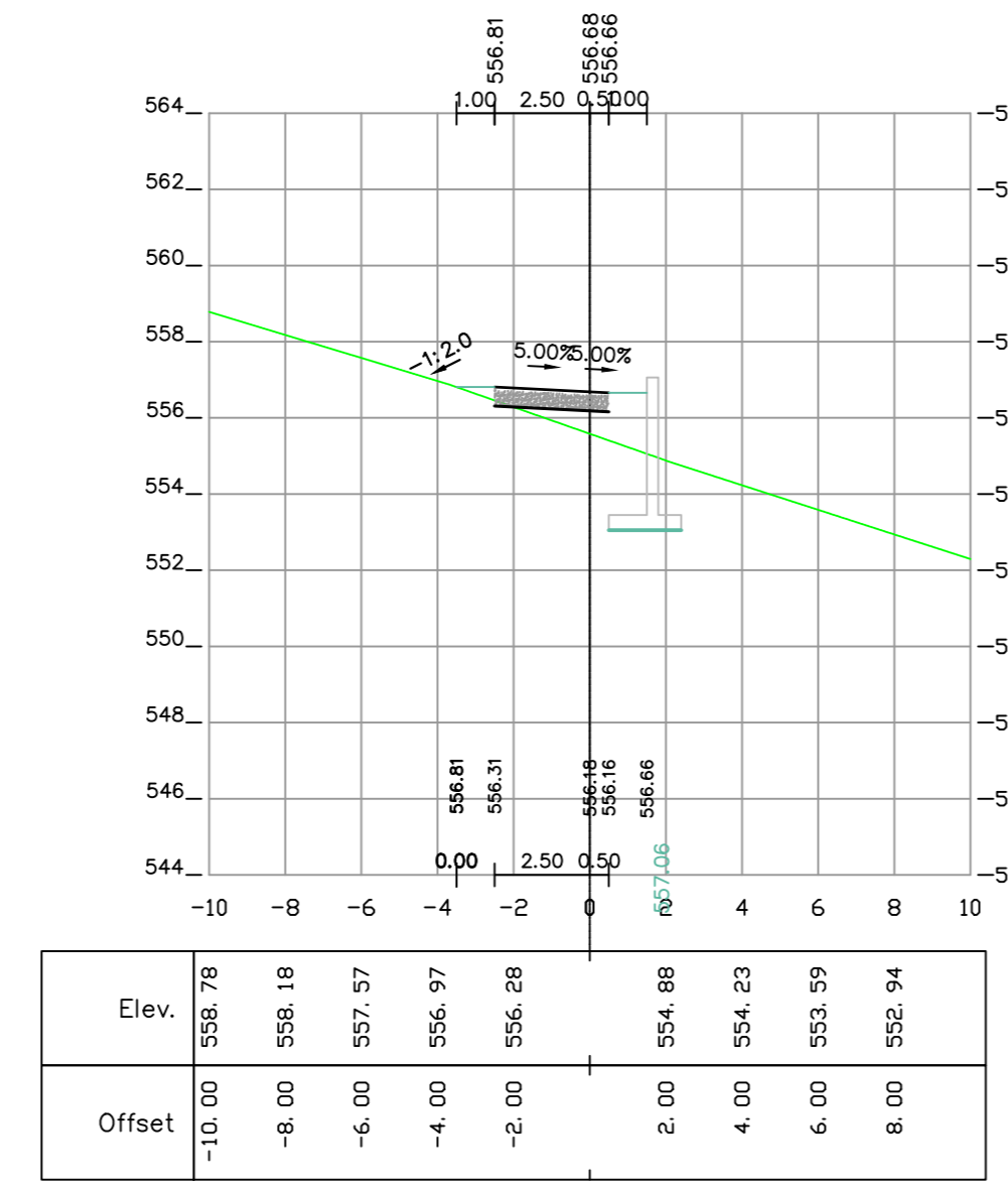
1+320 [Road road-3]
