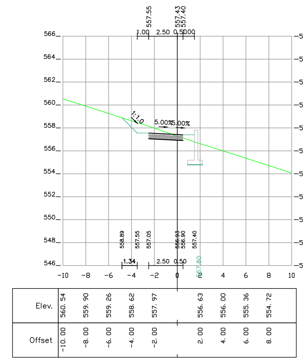
1+340 [Road road-3]
