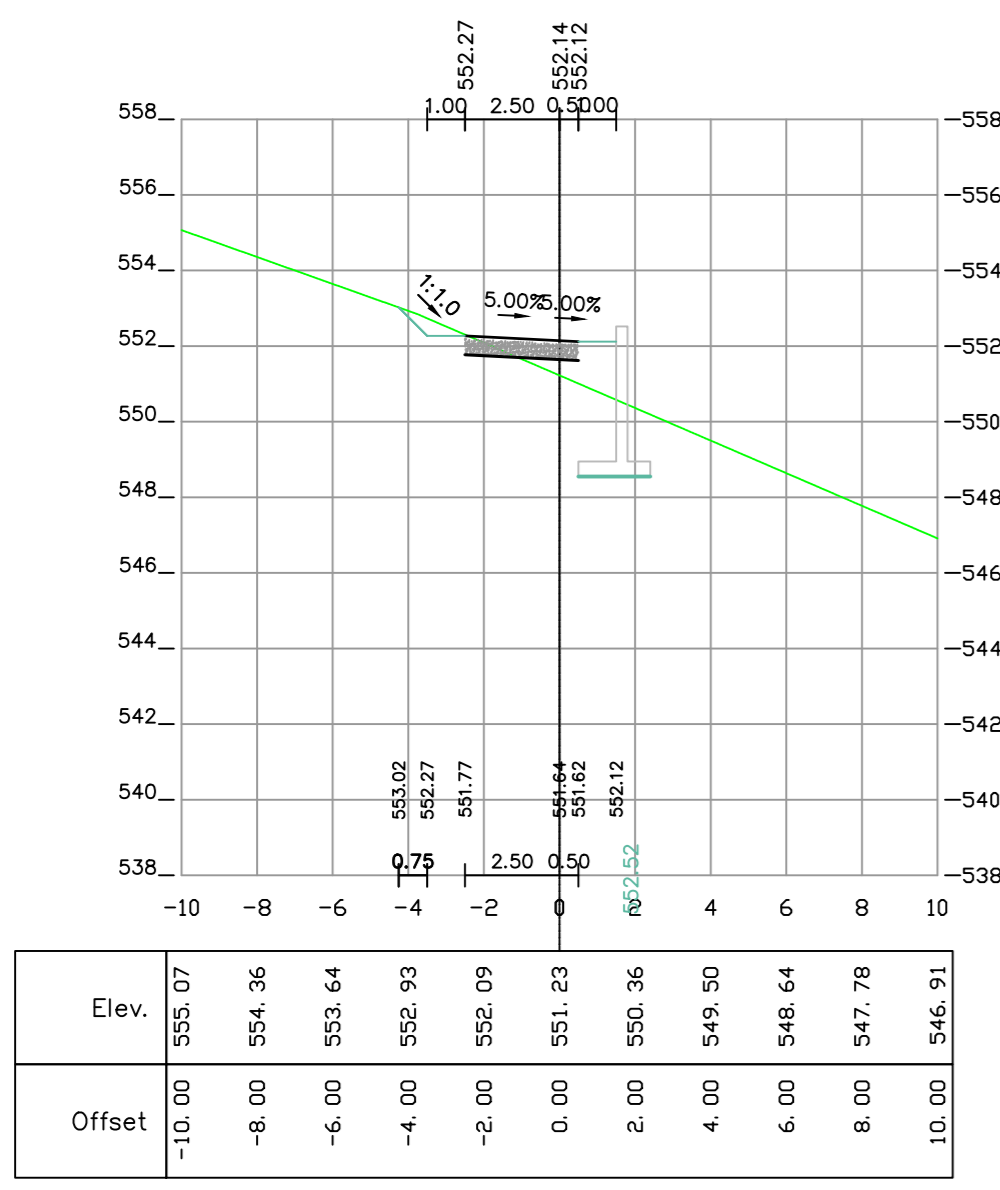
1+180 [Road road-3]
