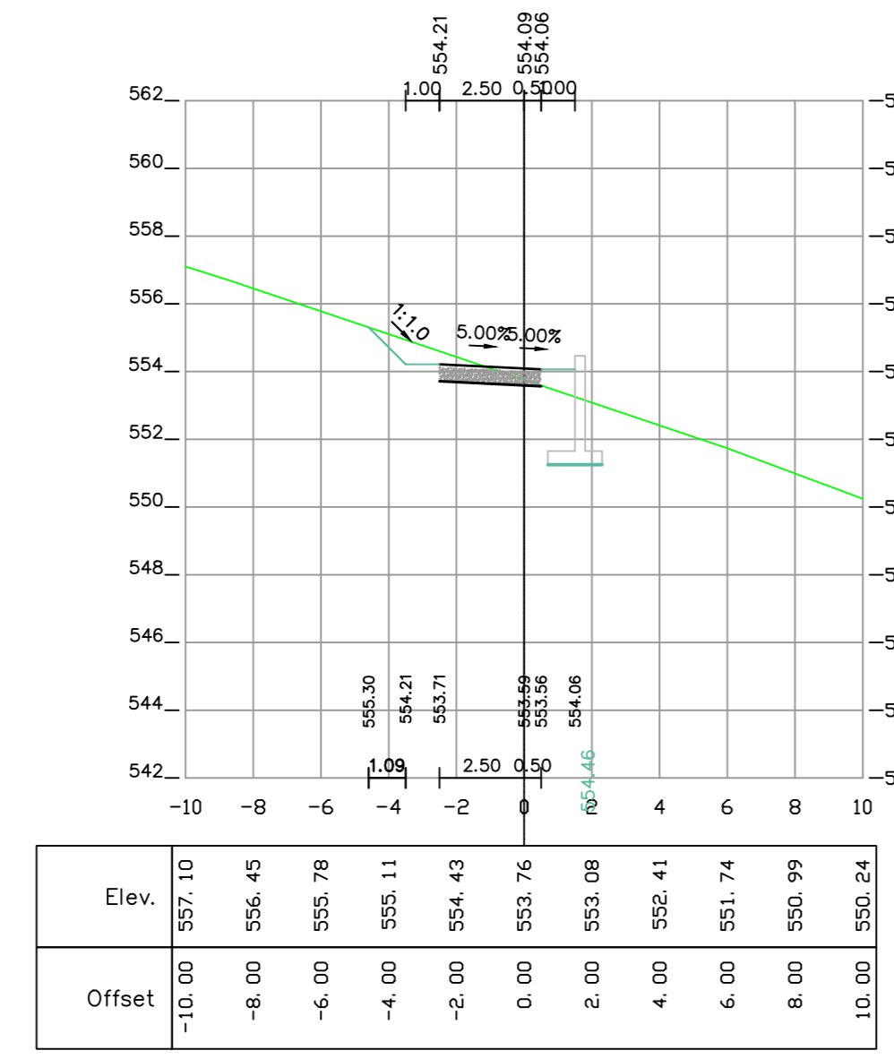
1+240 [Road road-3]
