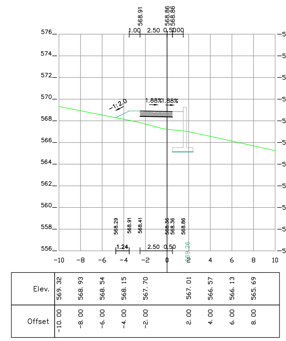
1+420 [Road road-3]
