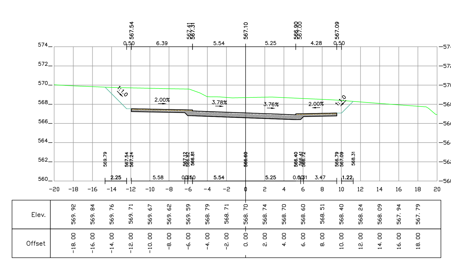
0+280 [Road 1]
