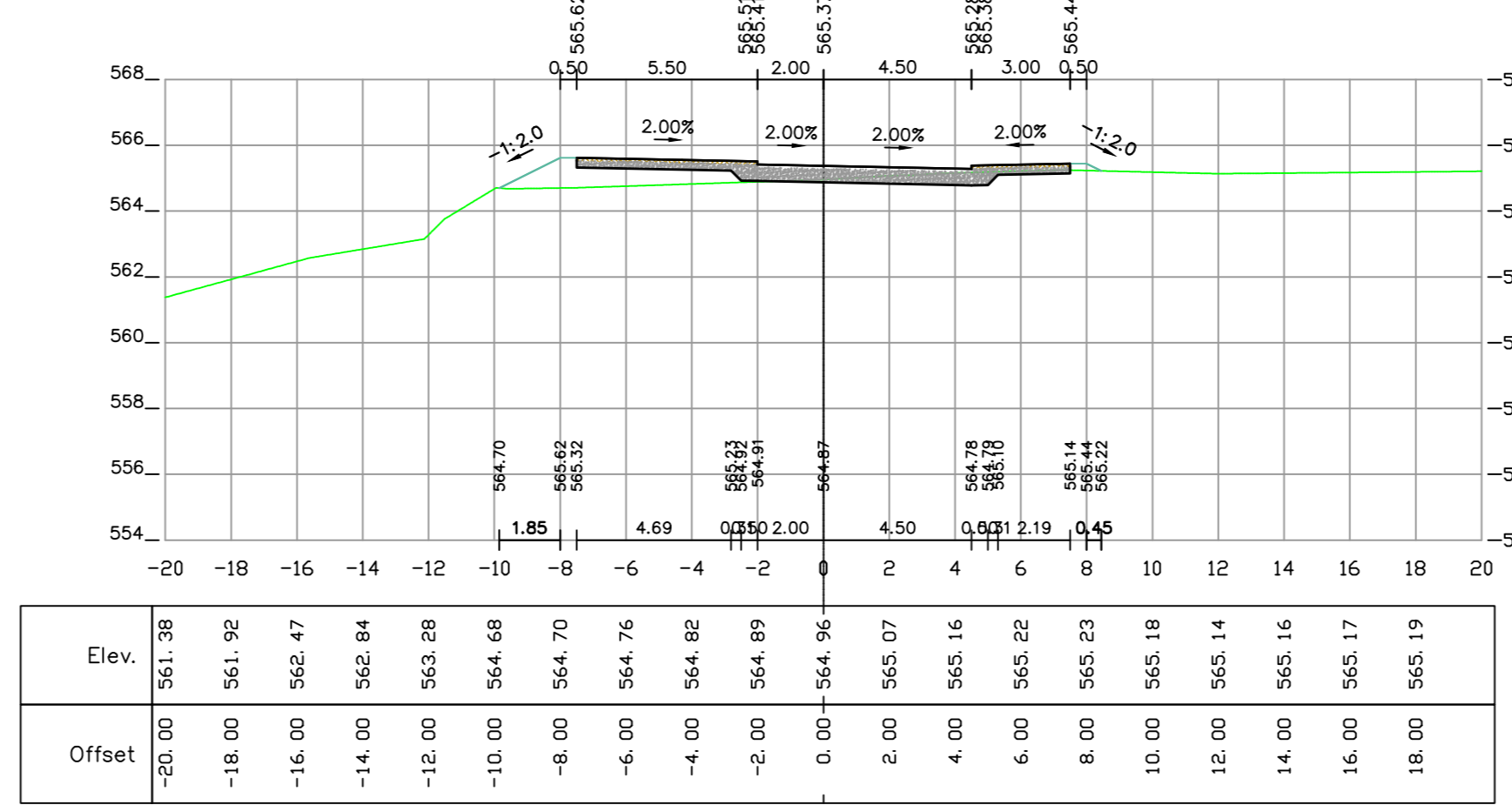
0+140 [Road 1]
