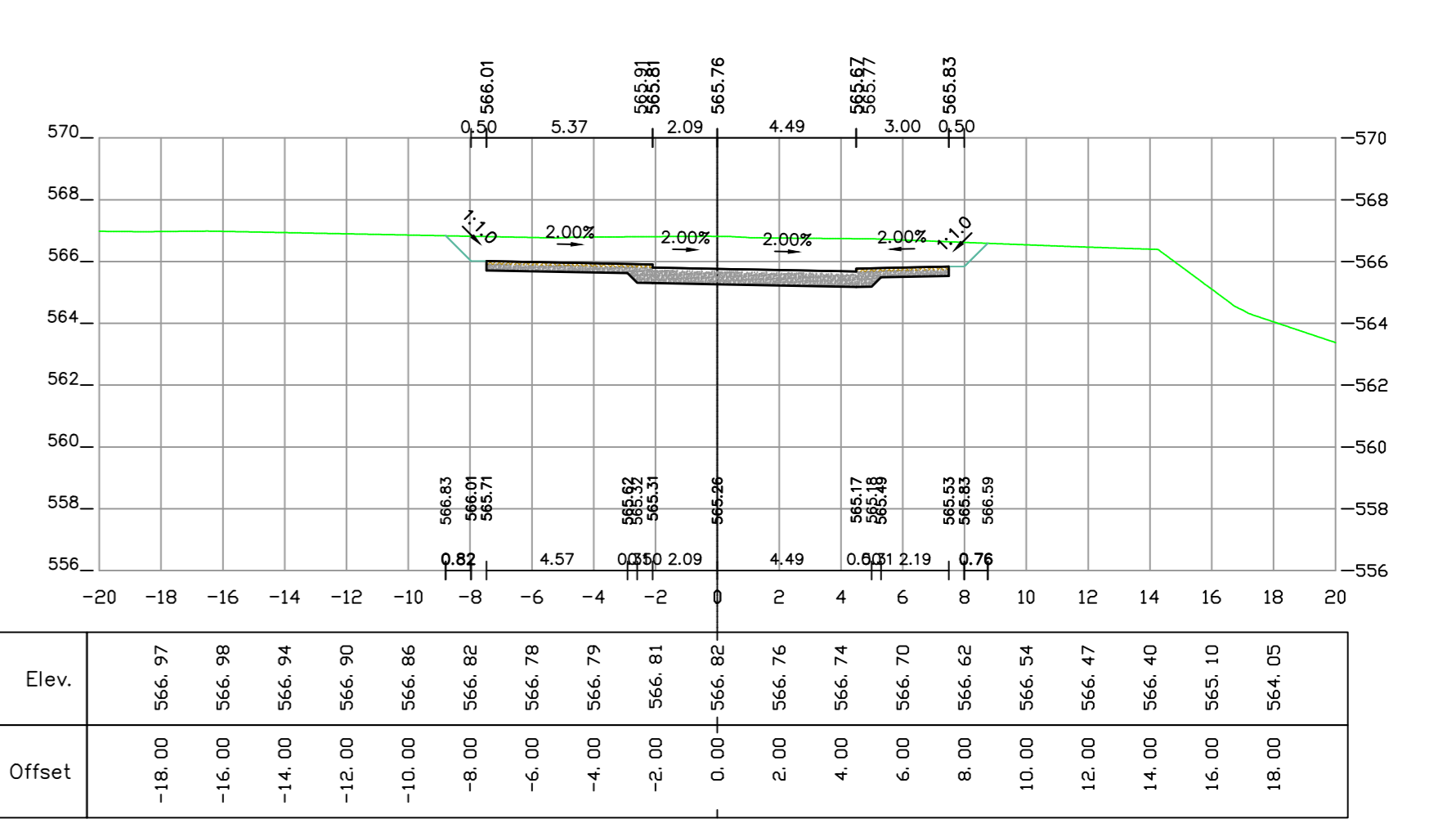
0+260 [Road 1]
