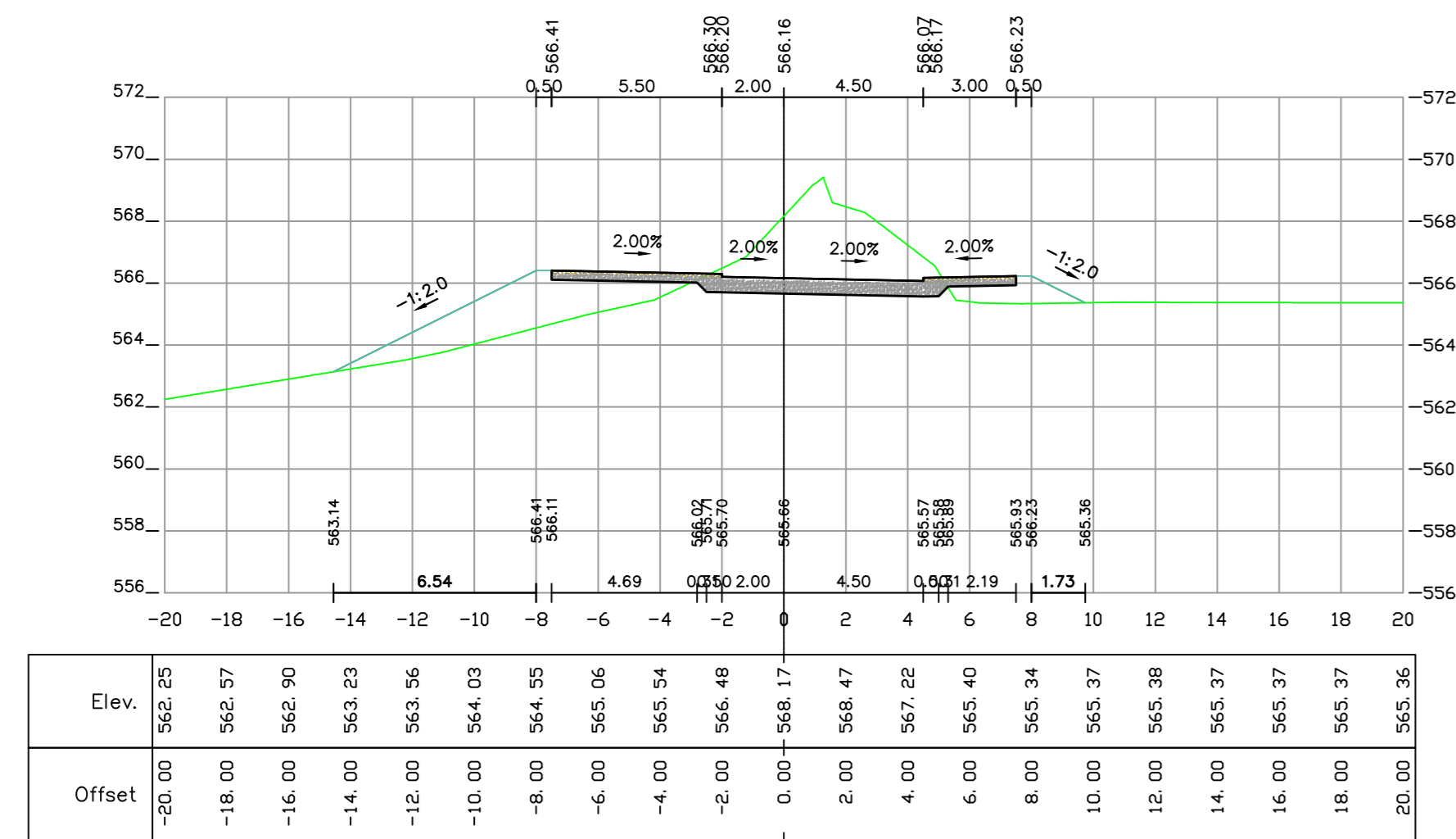
0+120 [Road 1]
